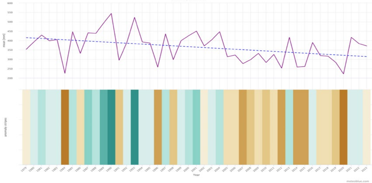
Mean yearly precipitation, trend and anomaly, 1979–2023. 49.42°N, 46.85°E.
