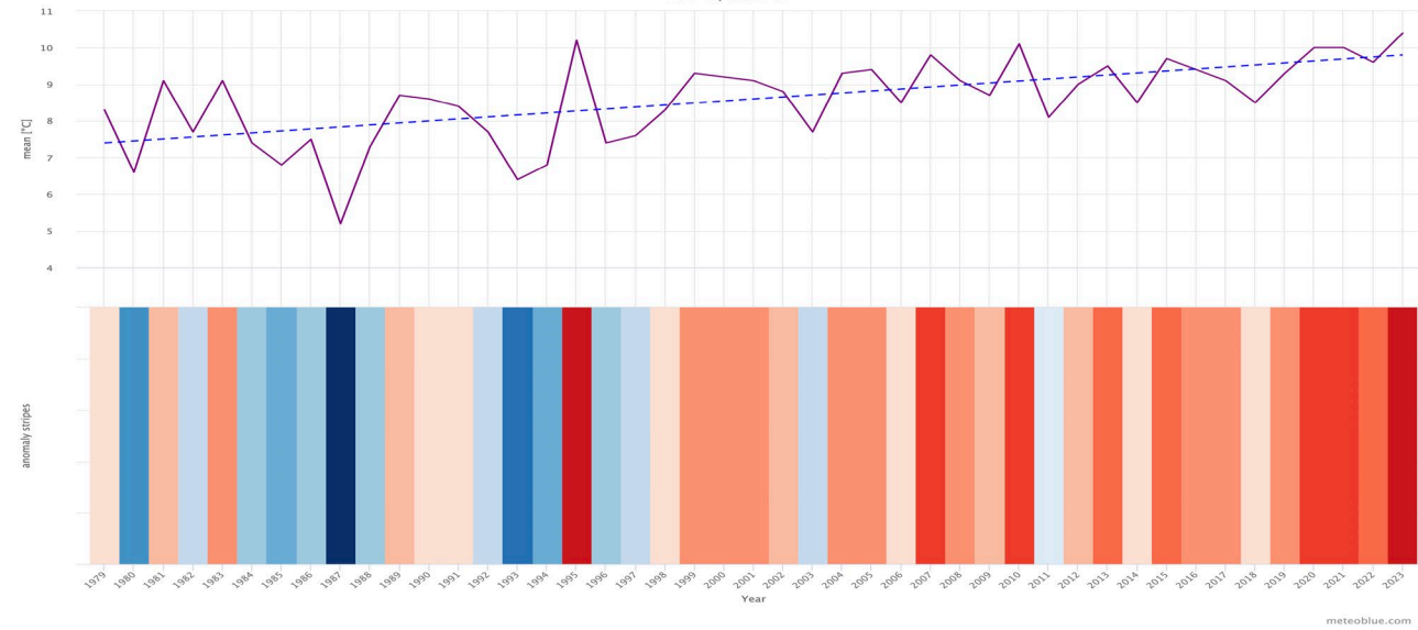
Mean yearly temperature, trend and anomaly, 1979–2023. 49.42°N, 46.85°E.
